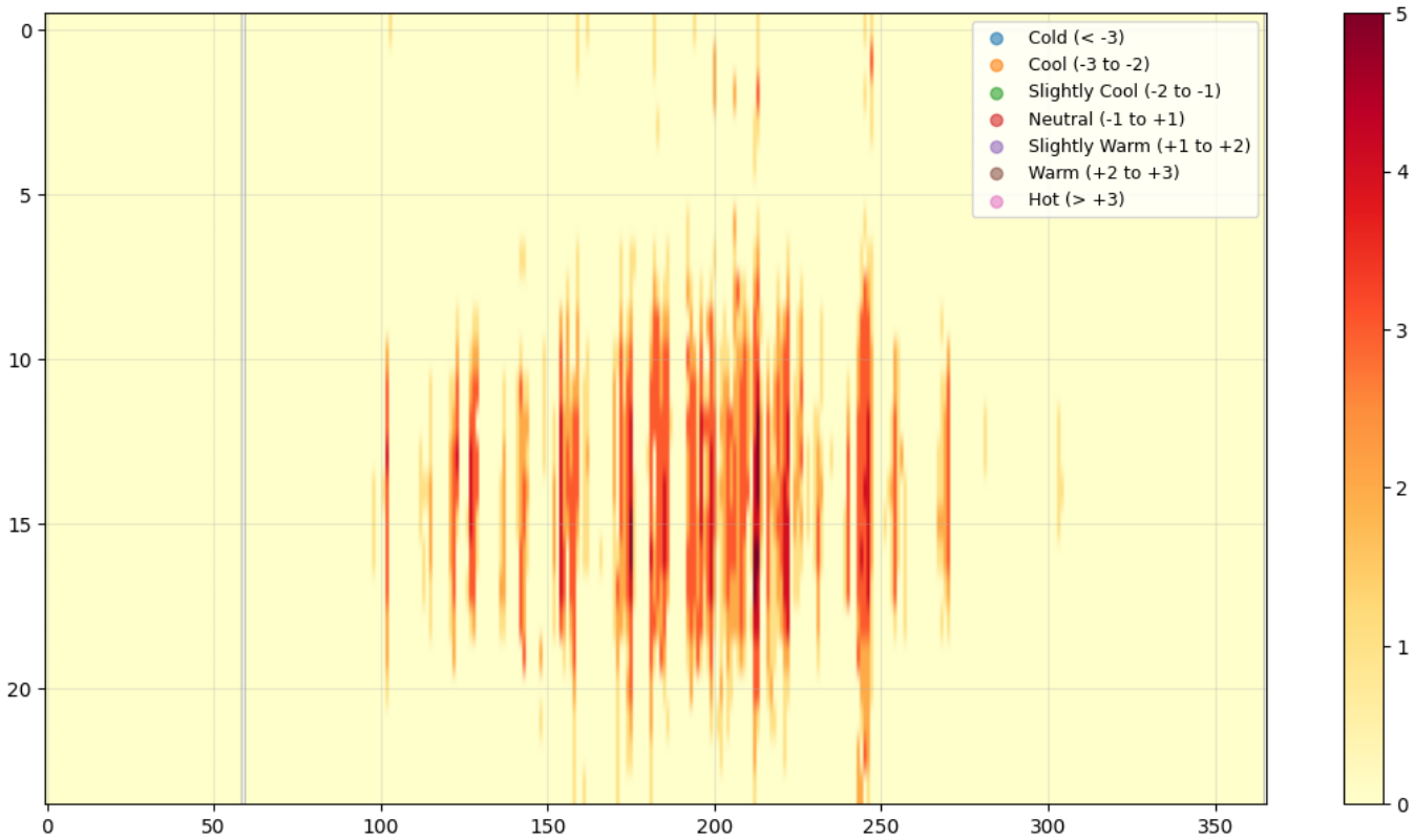
PMV_INDEX ANNUAL HEATMAP
