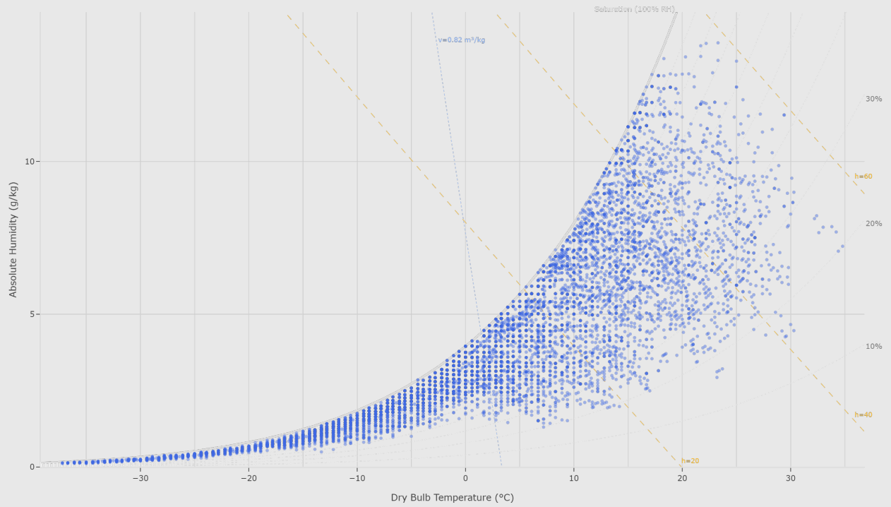
Psychrometric Chart
