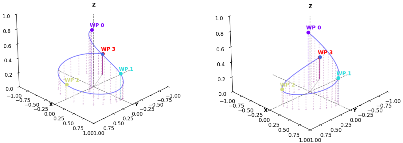
Figure 4: Joint space (left) vs task space (right) interpolation
