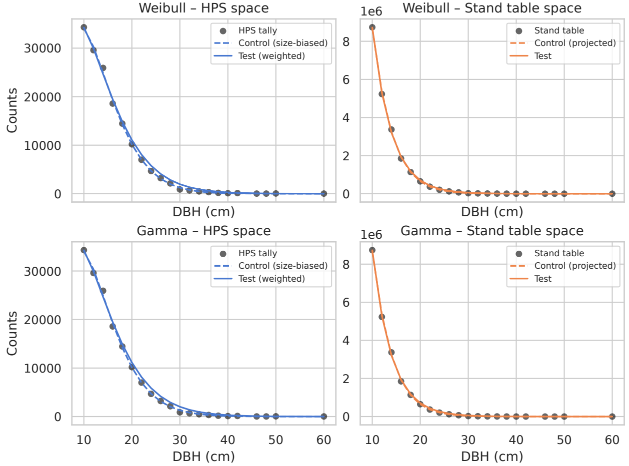
Fig. 1 Example comparison of control (size-biased) and test (weighted) estimators for the SPFL-S meta-plot. Solid lines denote weighted fits and dashed lines denote size-biased fits. Points represent empirical data (expanded stand tables on the right panels). Remaining combinations are supplied as supplementary figures
