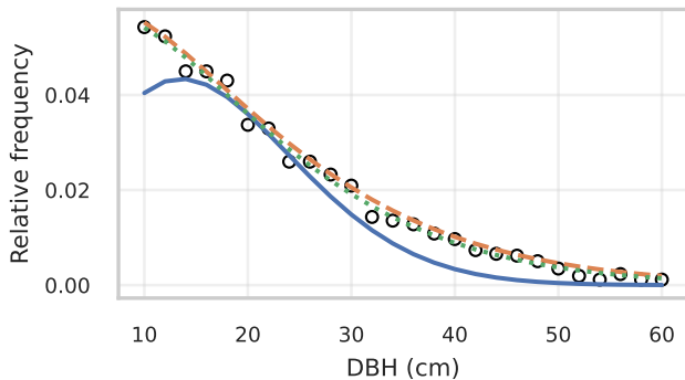
Weibull
