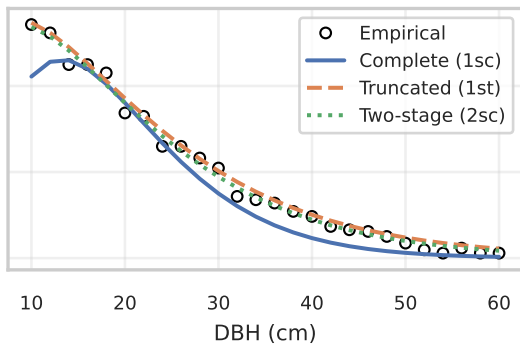
Gamma
