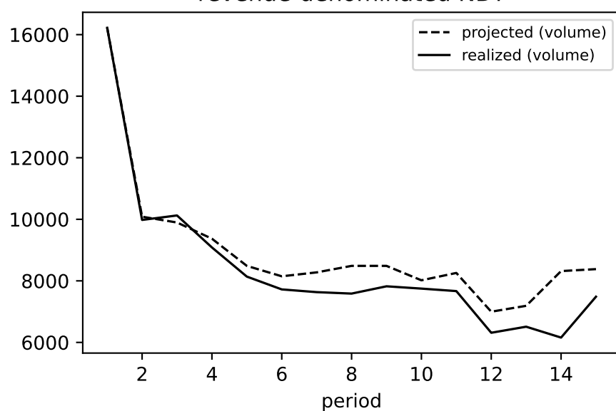
revenue-denominated NDY
