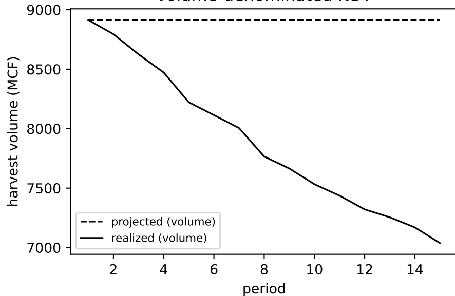
volume-denominated NDY
