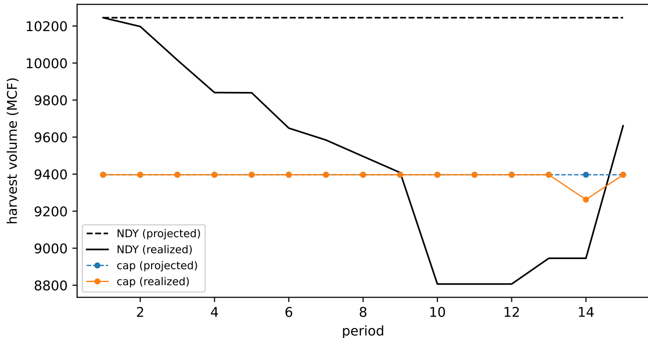
Landbase 1 at 4%: NDY flow link vs calibrated max-harvest cap
