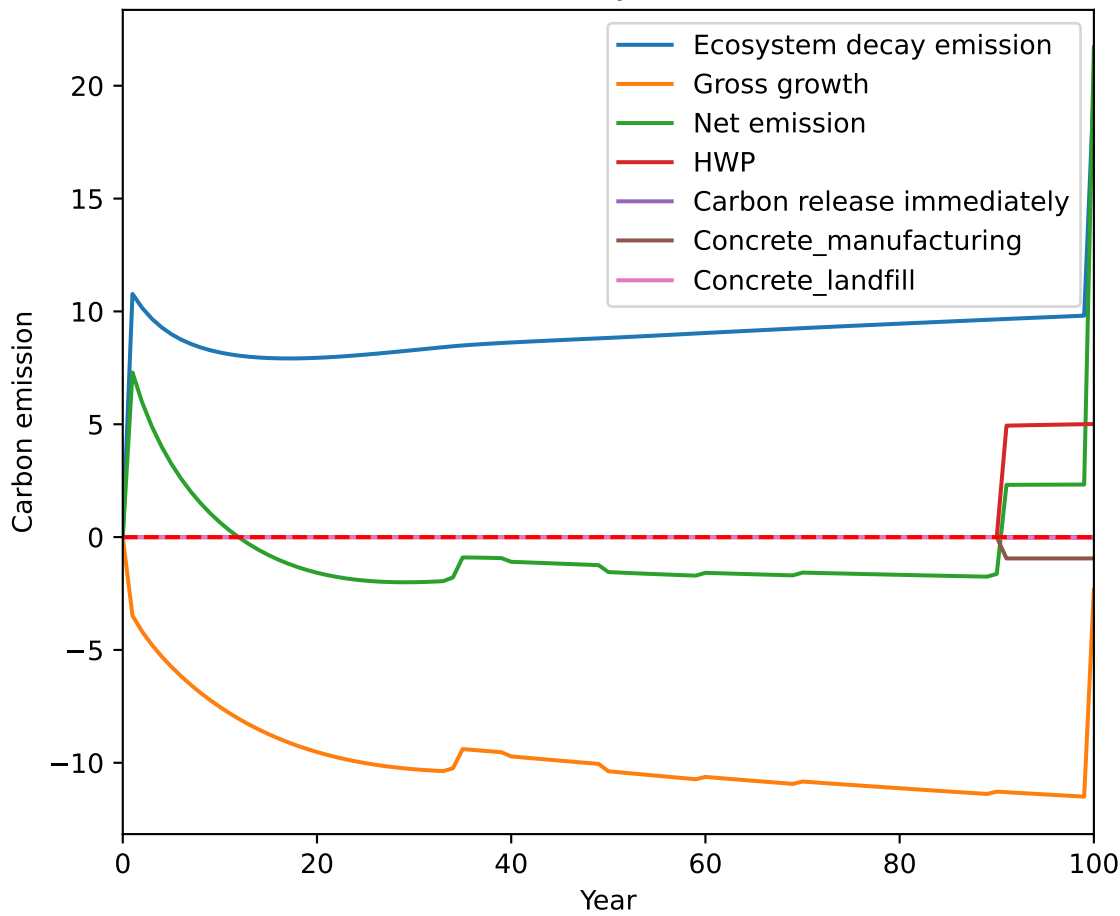
Carbon emission over years (base scenario)
