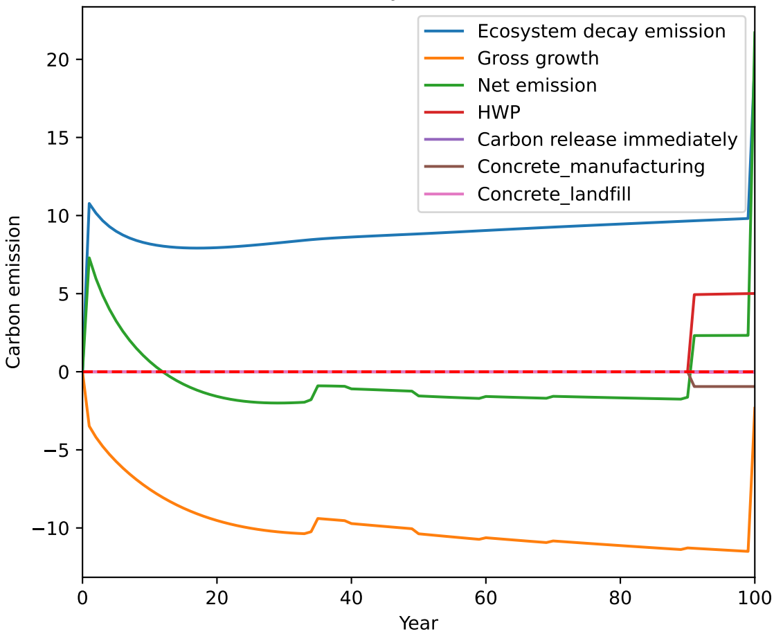
Carbon emission over years (alternative scenario)
