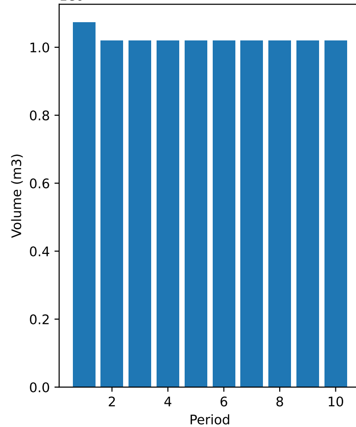
Harvested volume
