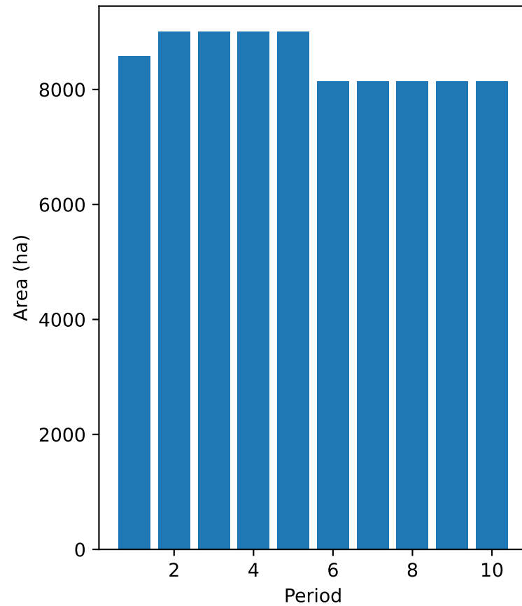
Harvested area
