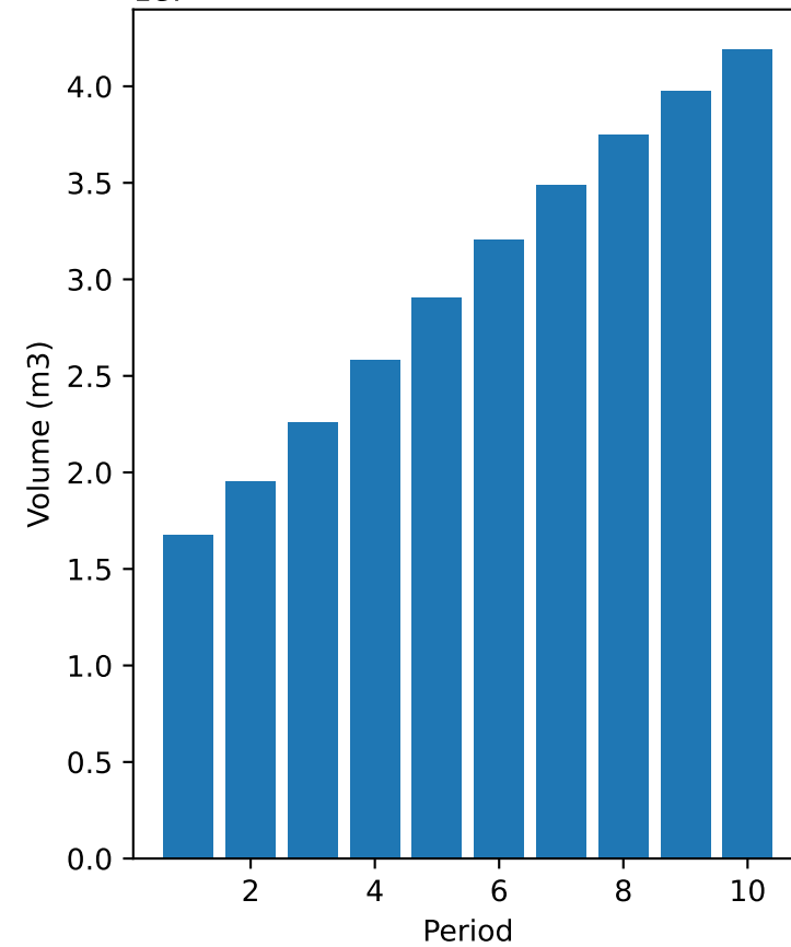
Growing Stock
