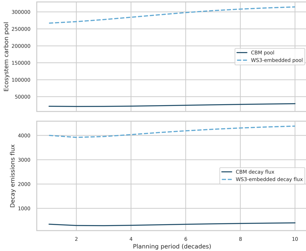
Figure 6: Neilson-hack demonstration (Example 040): comparison of libCBM (solid) and WS3-embedded (dashed) carbon indicators after bootstrapping pools/fluxes into WS3 as yield curves. Top: ecosystem carbon pools; Bottom: aggregate decay emissions flux.
