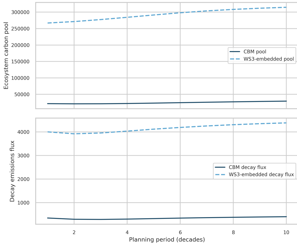
Figure 9: Neilson-hack demonstration (Example 040): comparison of libCBM (solid) and WS3-embedded (dashed) carbon indicators after bootstrapping pools/fluxes into WS3 as yield curves. Top: ecosystem carbon pools; Bottom: aggregate decay emissions flux.
