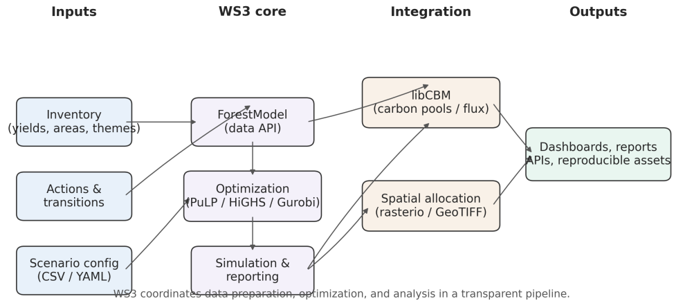
Figure 1: WS3 architecture: inputs feed a ForestModel; scenarios are scheduled via heuristic or LP; results feed libCBM and optional spatial allocation; plots/tables generated for analysis.
