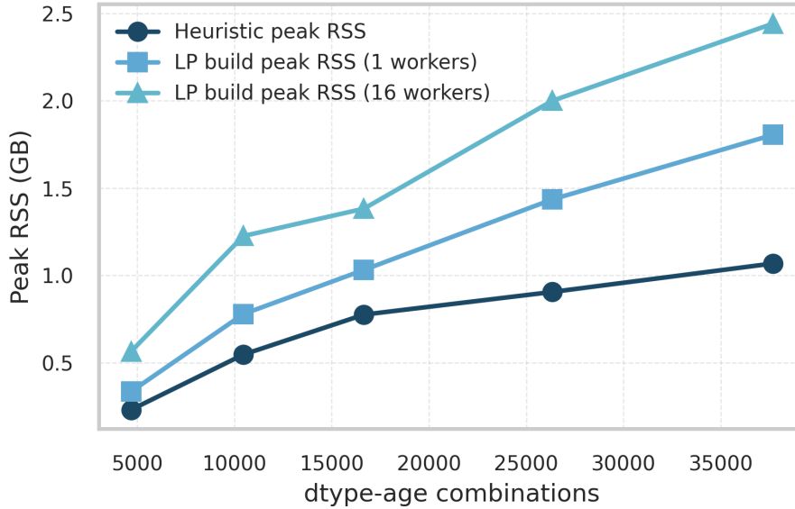
Figure 6: Peak resident memory for heuristic scheduling (serial) and LP model builds (1 and 16 workers).
