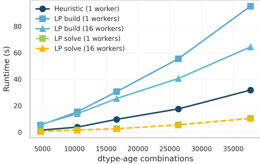
Figure 4: Scheduling runtime versus problem size. Heuristic runs are single worker; LP build/solve lines appear when RUN_LP=1 .
