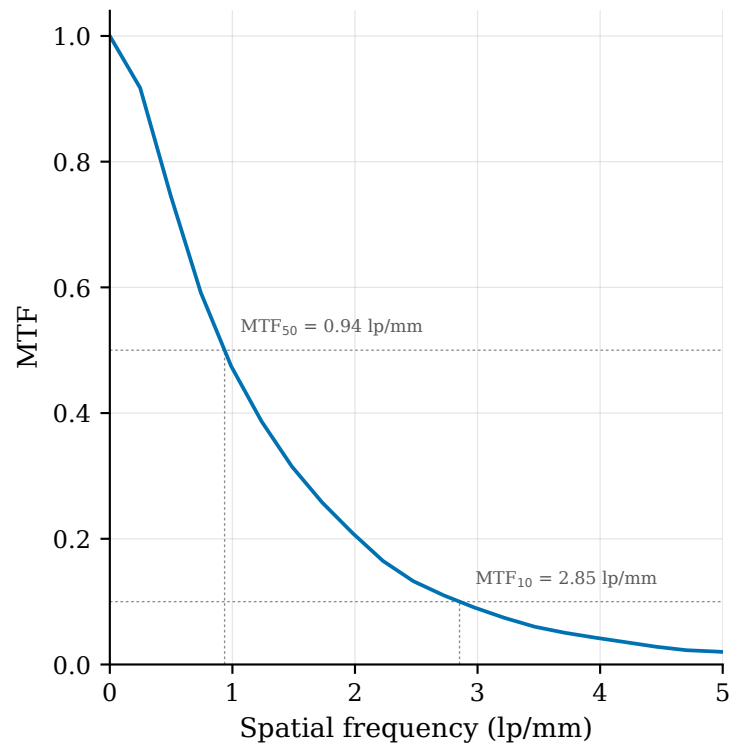
MTF
