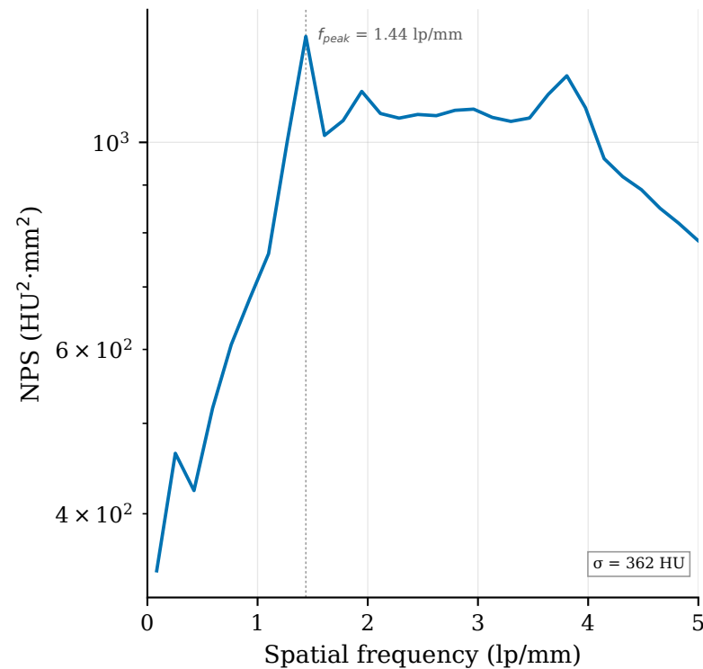
NPS
