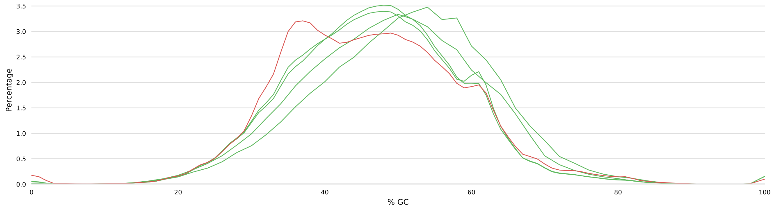
FastQC: Per Sequence GC Content
