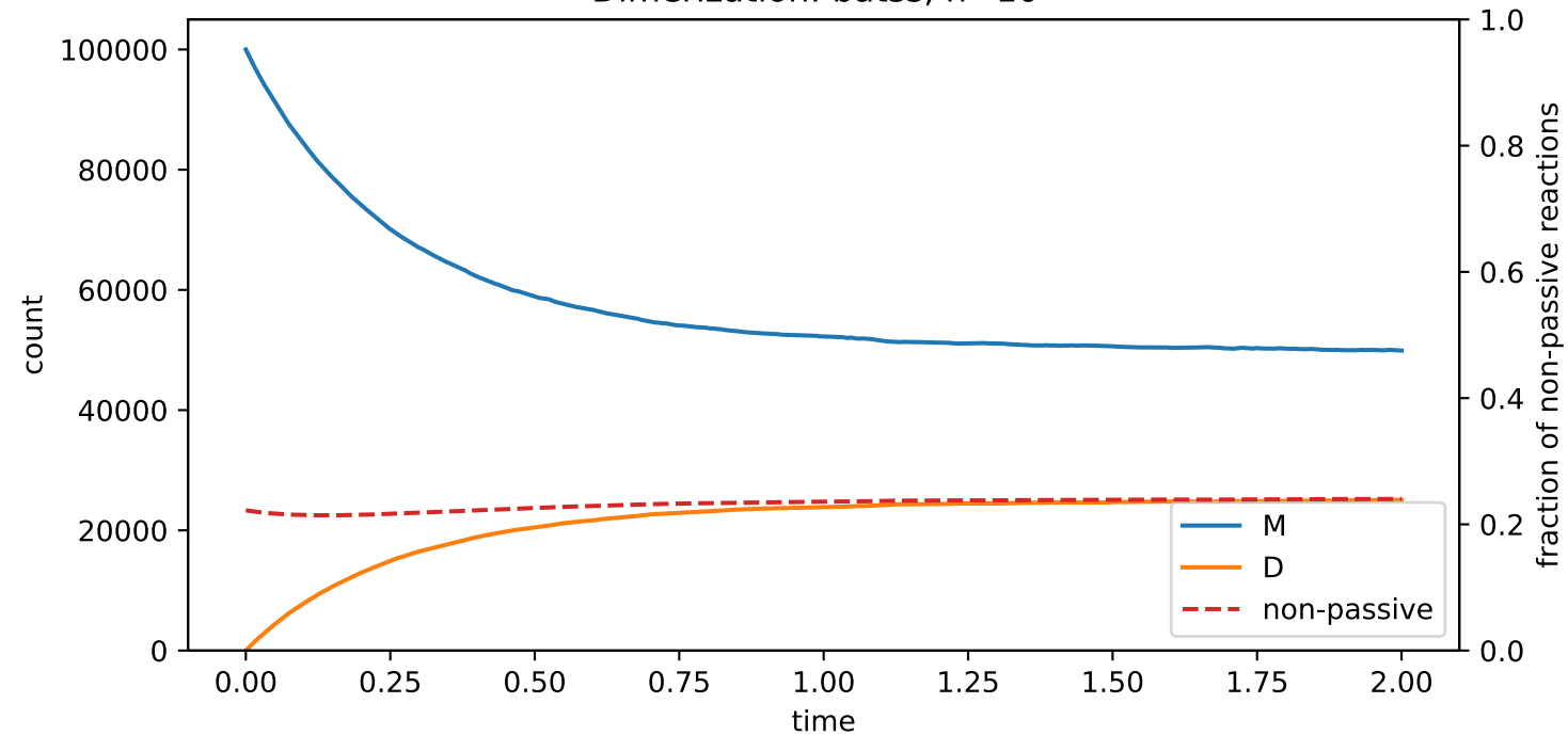
Dimerization: batss, n=10^5
