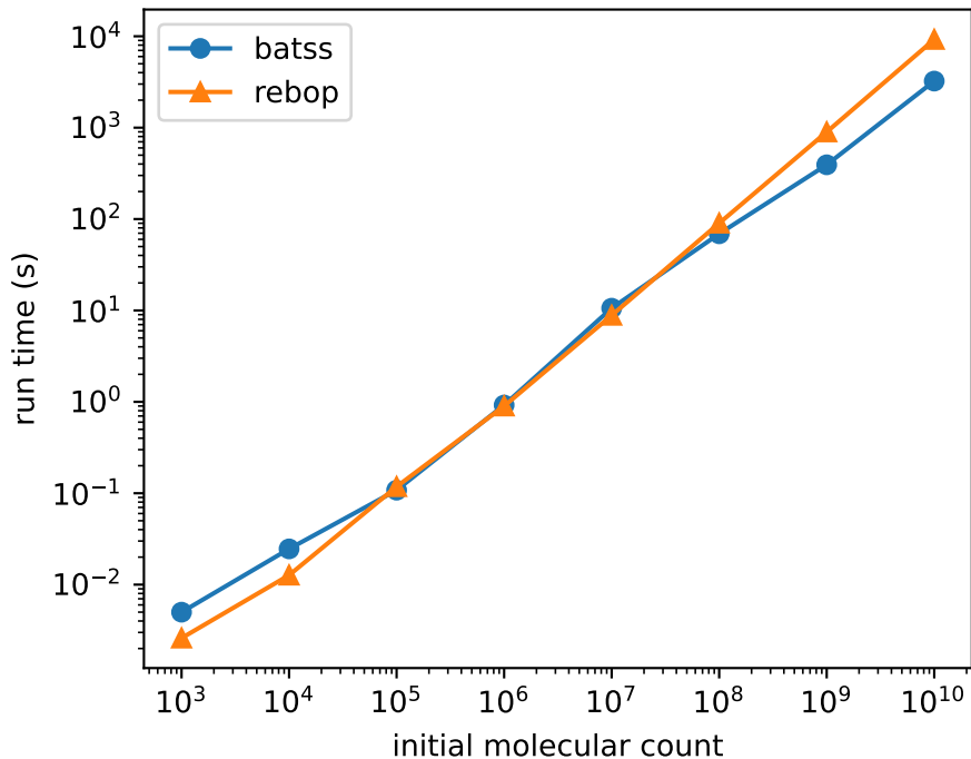
Oregonator: run time to simulate t=1.0
