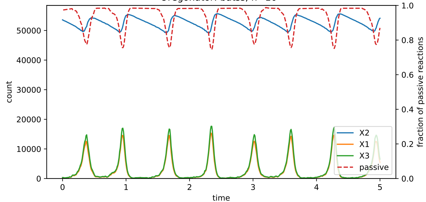
Oregonator: batss, n=10^5
