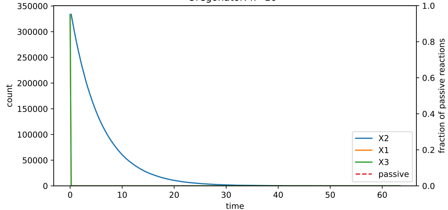
Oregonator: n=10^6
