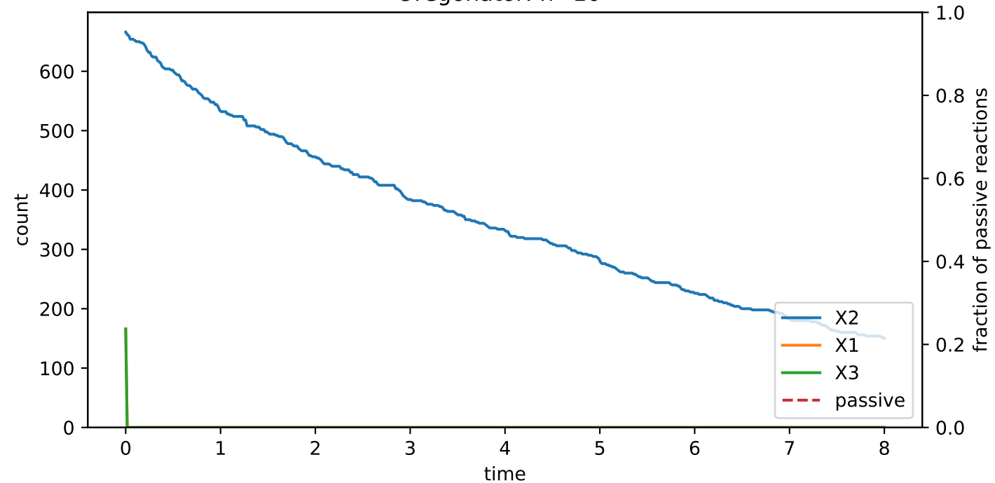
Oregonator: n=10^3
