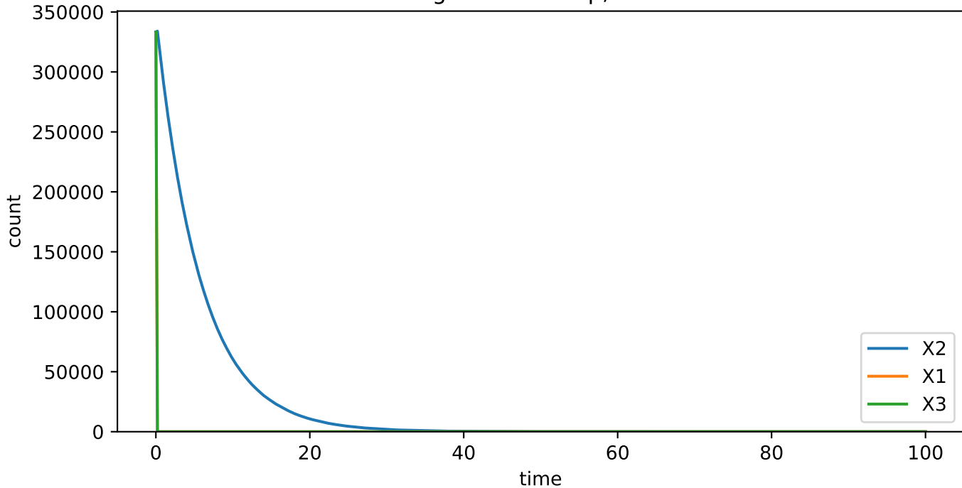
Oregonator: rebop, n=10^6
