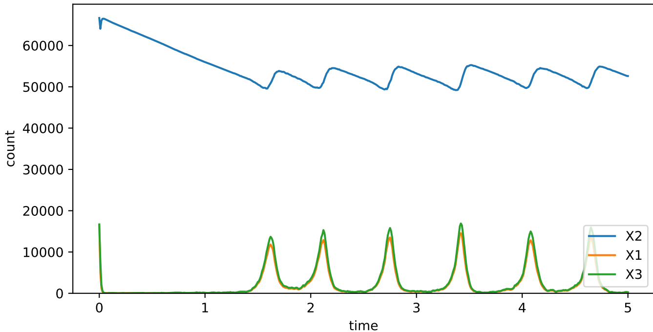
Oregonator: rebop, n=10^5
