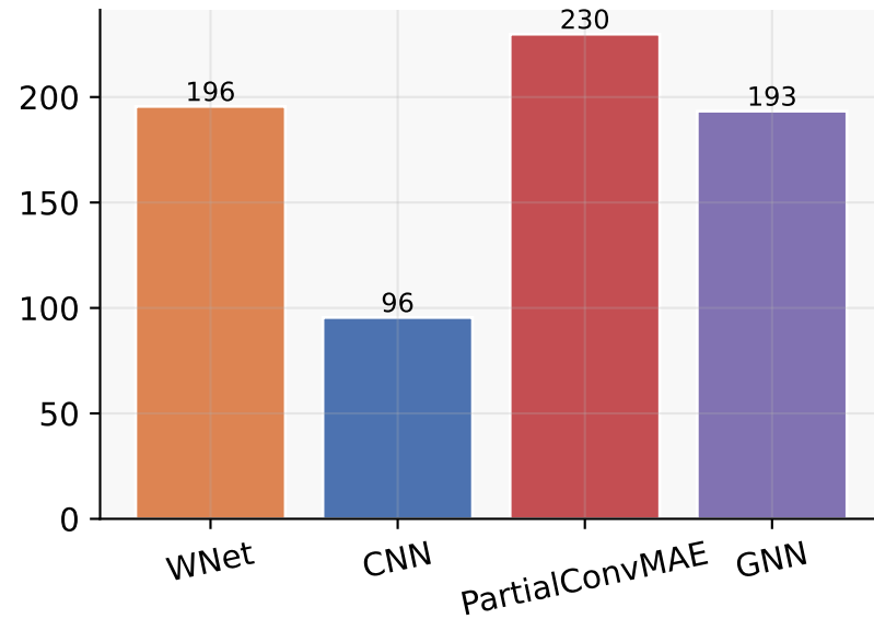
Mean Steps per Episode
