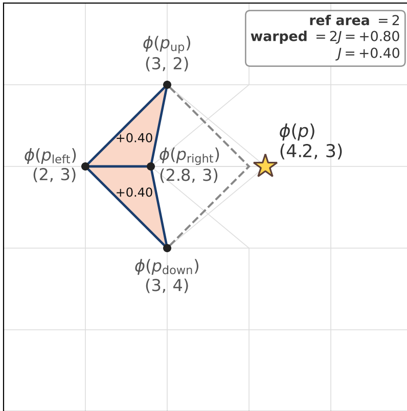
(b) Central differences: 4-neighbour diamond, two triangles
