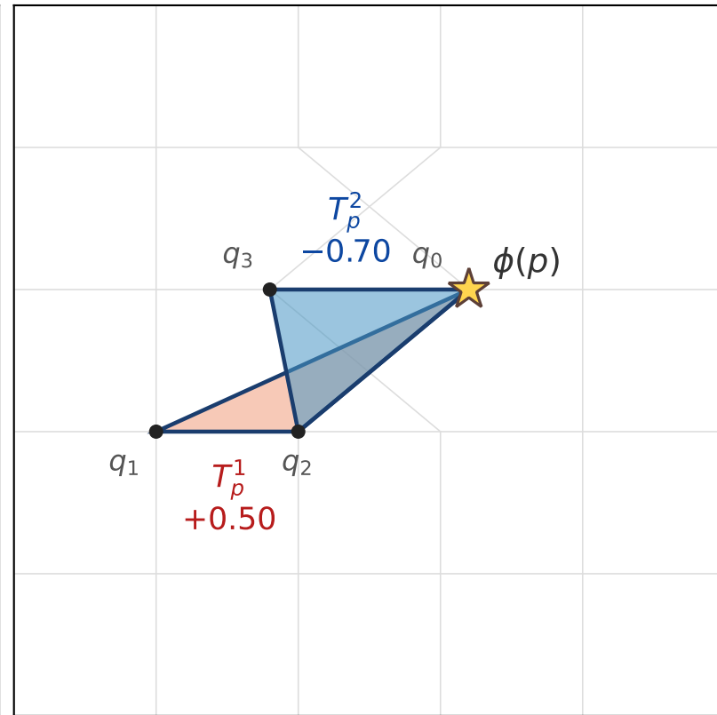
(c) Two-triangle check at p : shared edge \overline{q_0 q_2}
