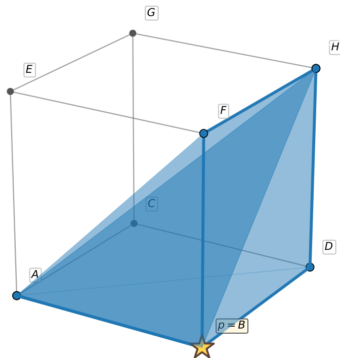
(b) -x source cell: anchored at p = B T_1 = [A, B, D, H] , T_2 = [A, B, F, H]
