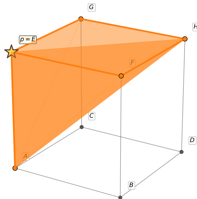
(d) -z source cell: anchored at p = E T_5 = [A, E, F, H] , T_6 = [A, E, G, H]
