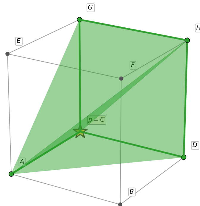
(c) -y source cell: anchored at p = C T_3 = [A, C, D, H] , T_4 = [A, C, G, H]
