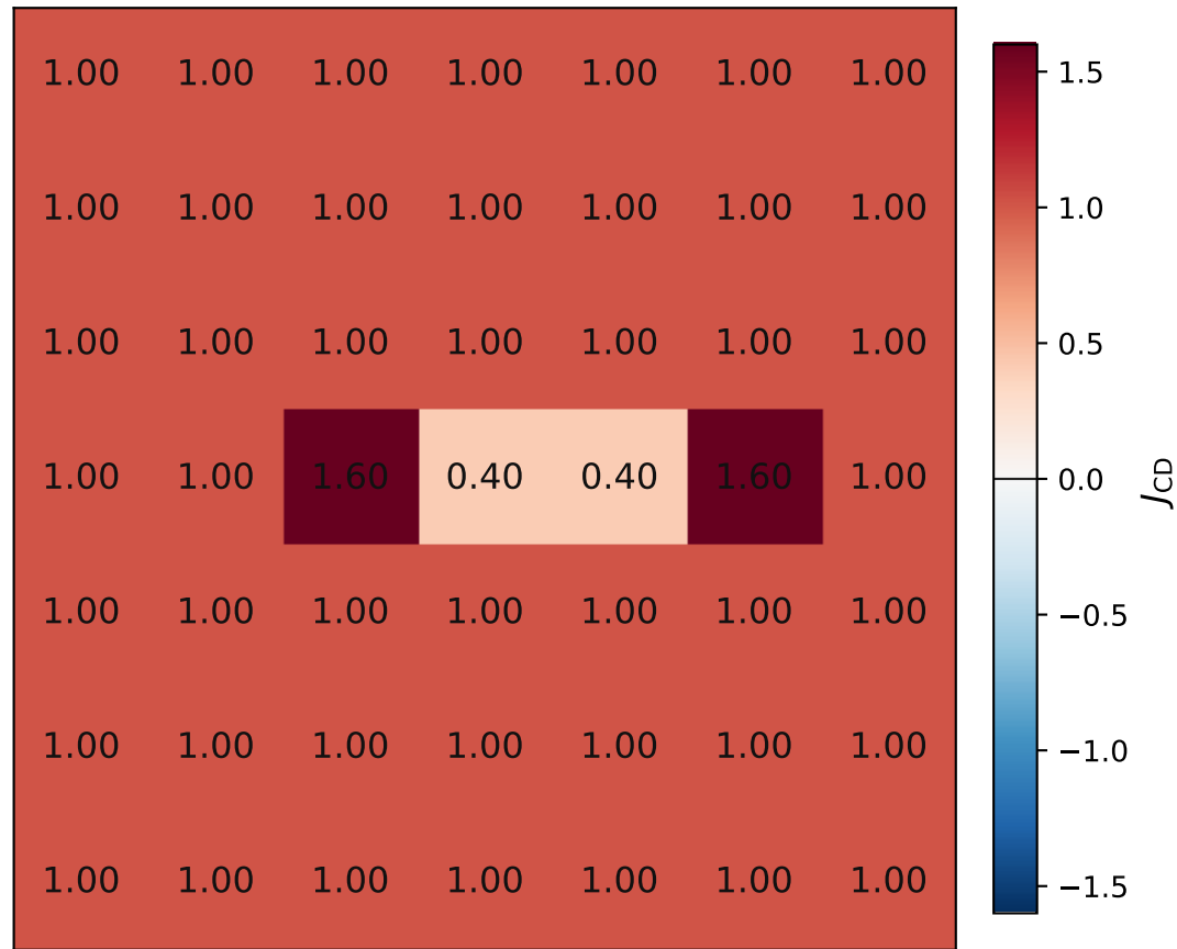
(c) J_{CD} of (b) - \min = 0.40 , no fold is detected
