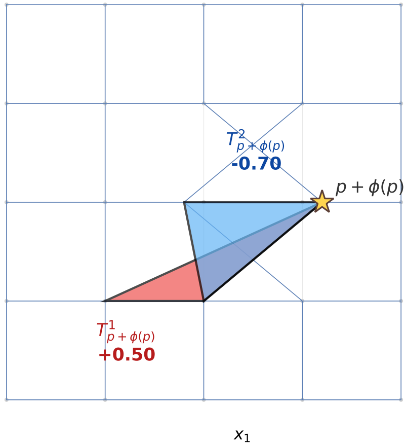
(b) Bowtie deformation
