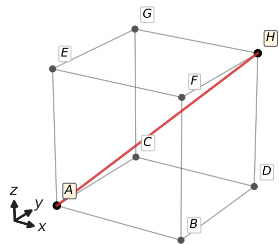
(a) Voxel cube + body diagonal \overline{AH}
