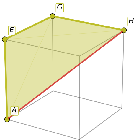
(g) T_6 = [A, E, G, H] , \text{vol}(T_6) = -\frac{1}{6}
