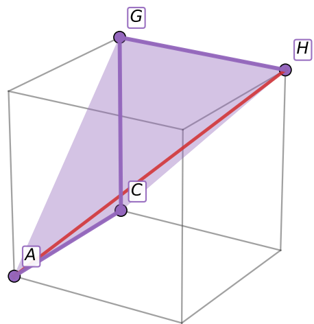
(e) T_4 = [A, C, G, H] , \text{vol}(T_4) = +\frac{1}{6}
