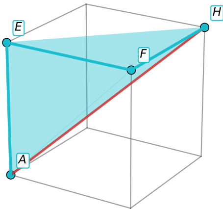
(f) T_5 = [A, E, F, H] , \text{vol}(T_5) = +\frac{1}{6}
