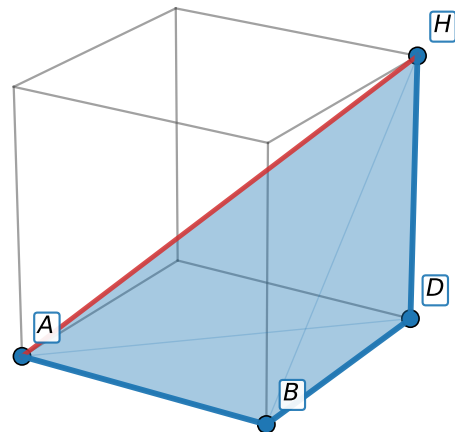
(b) T_1 = [A, B, D, H] , \text{vol}(T_1) = +\frac{1}{6}
