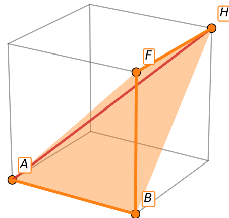
(c) T_2 = [A, B, F, H] , \text{vol}(T_2) = -\frac{1}{6}
