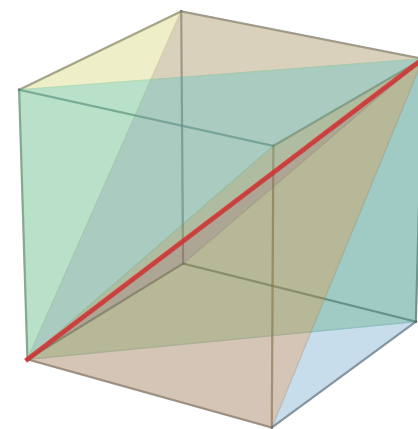
(h) All six tetrahedra stacked
