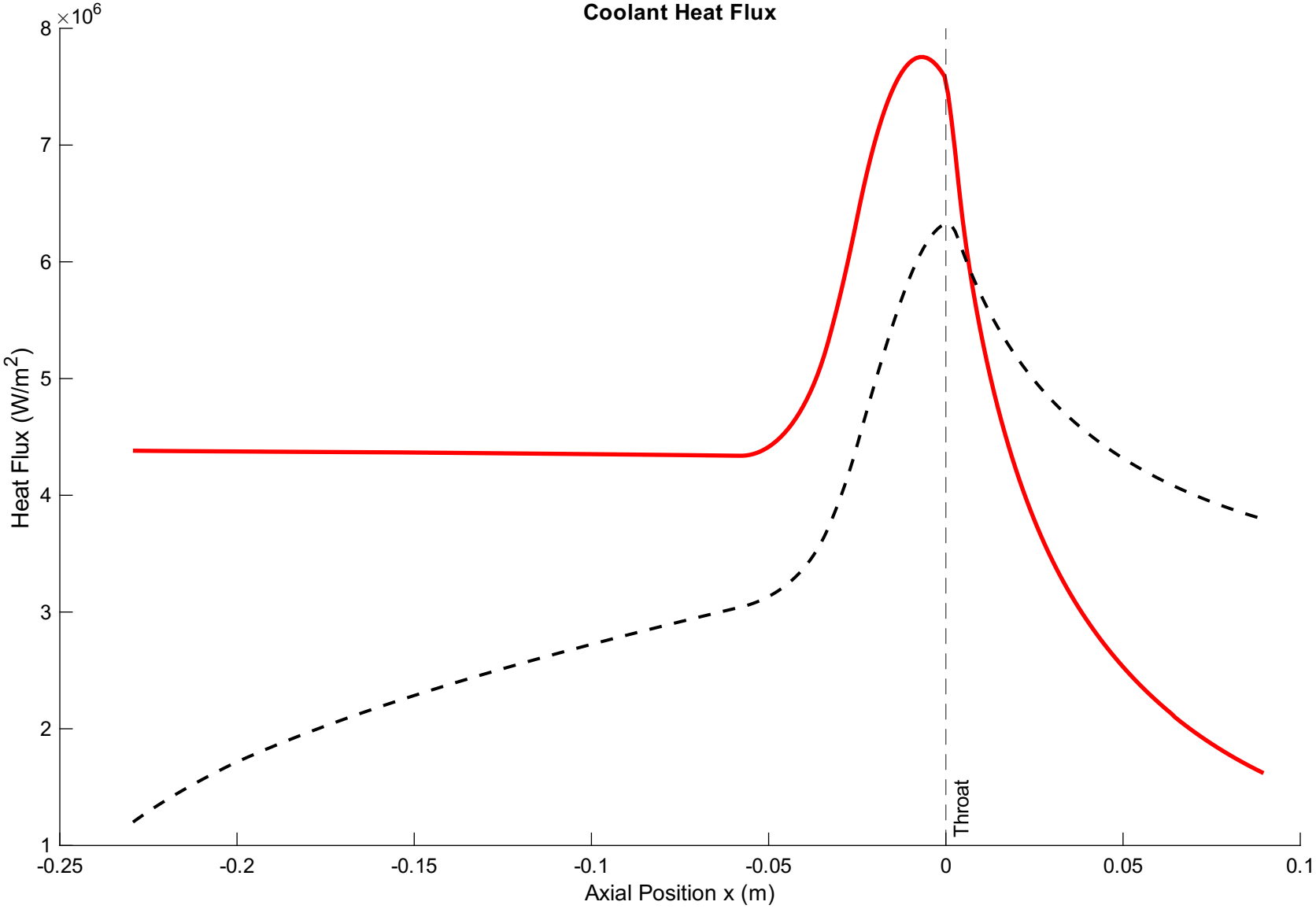
Coolant Heat Flux
