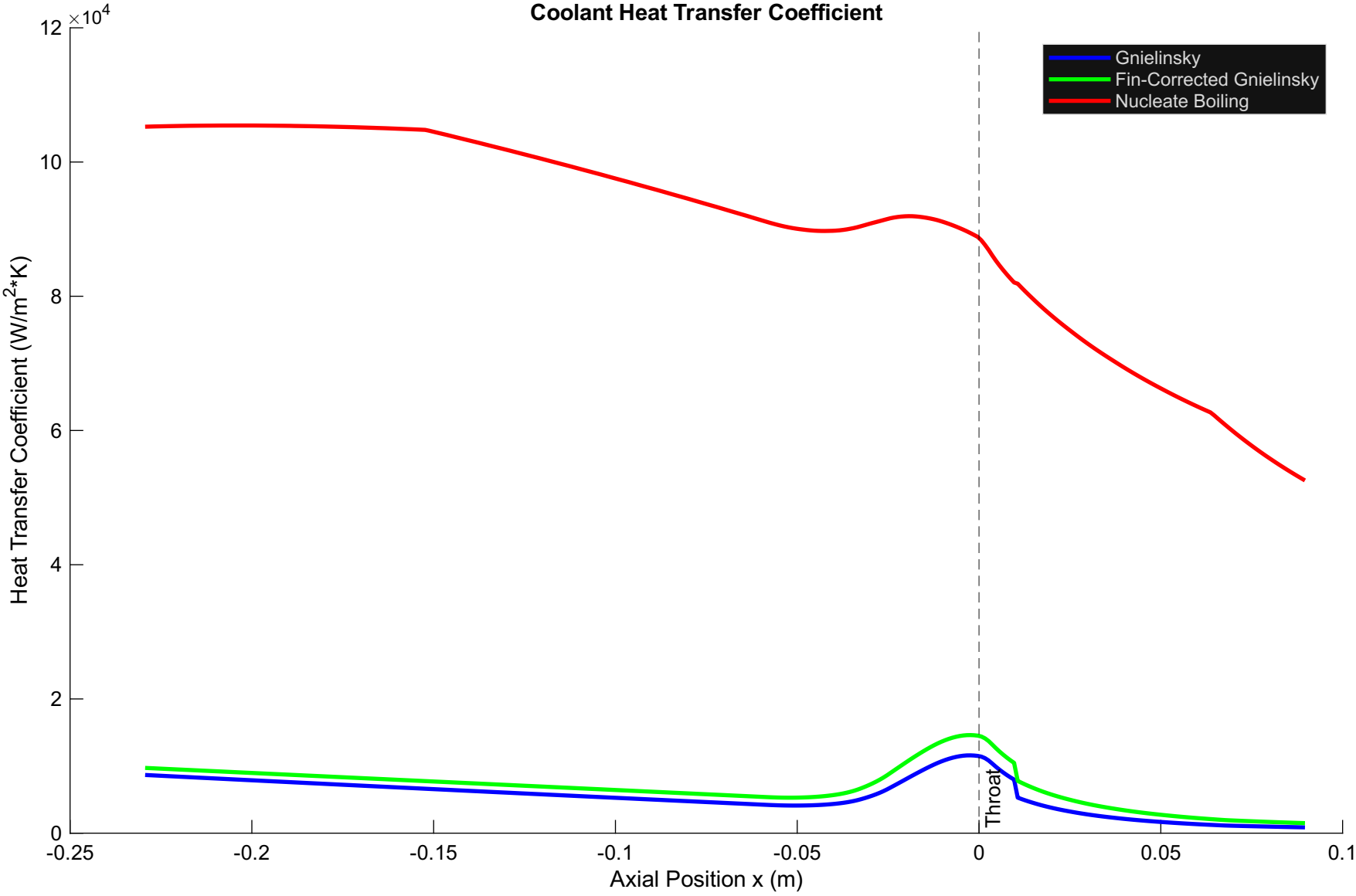
Coolant Heat Transfer Coefficient
