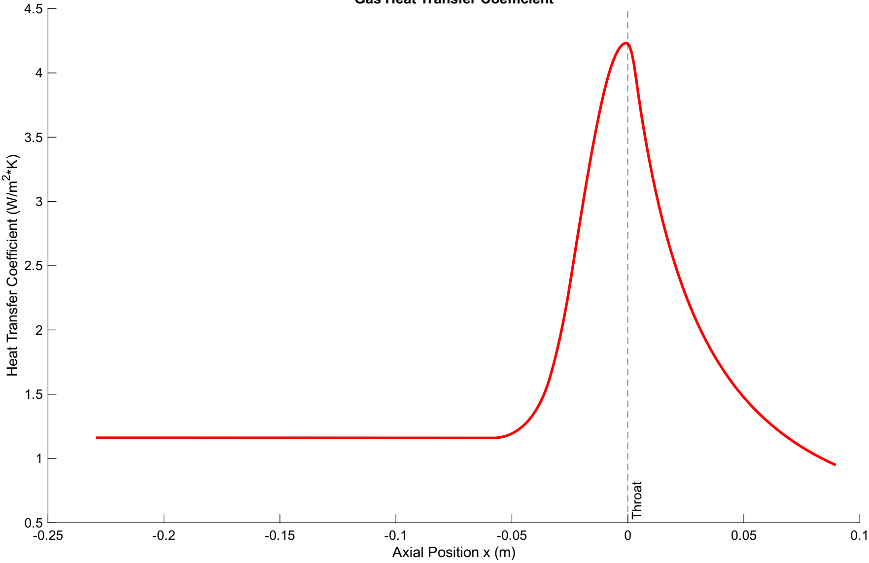
Gas Heat Transfer Coefficient
