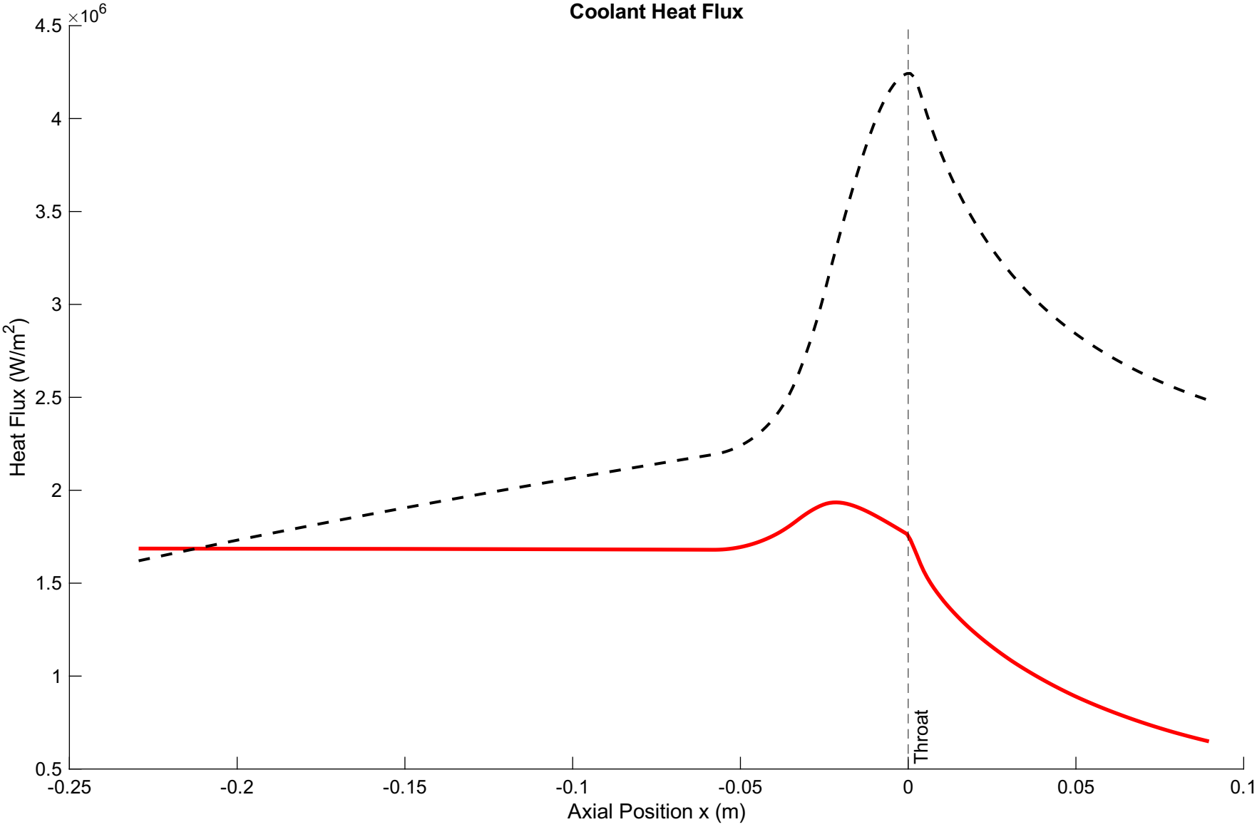
Coolant Heat Flux
