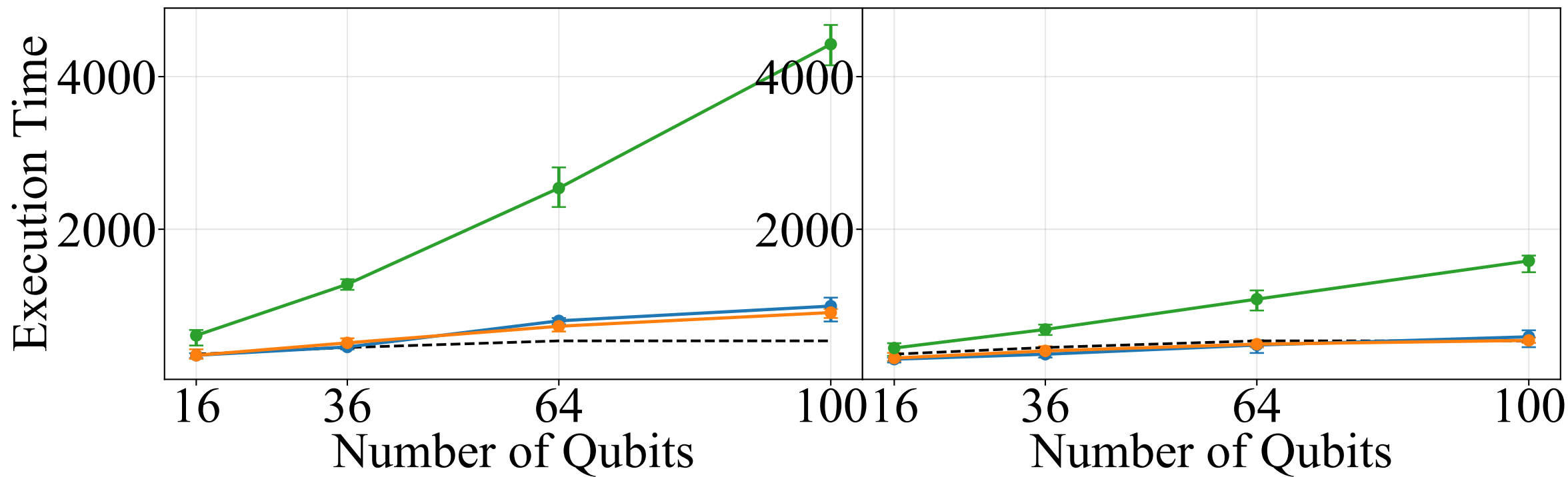
Microarchitecture Comparison AOD = 1 AOD = 5
