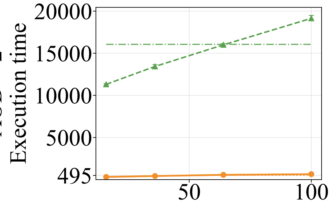
Full Trotter
