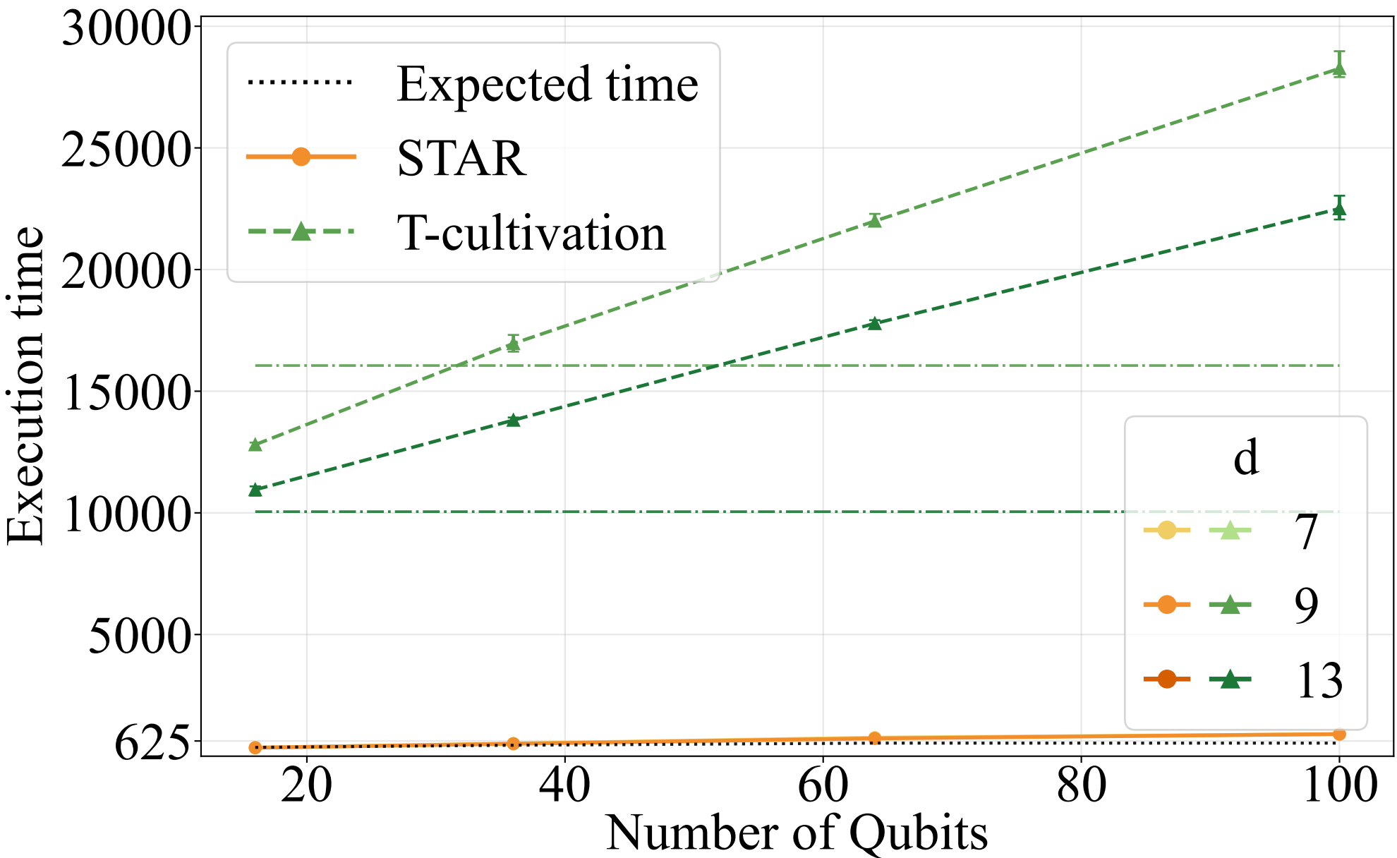
Overall execution time comparison: STAR vs T
