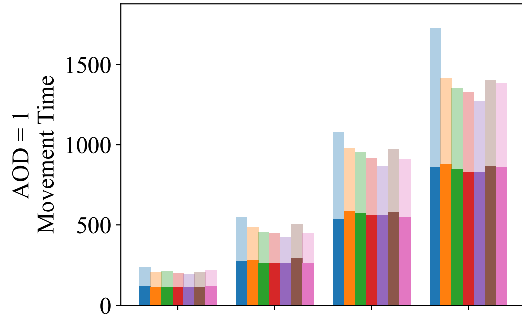
Full Trotter
