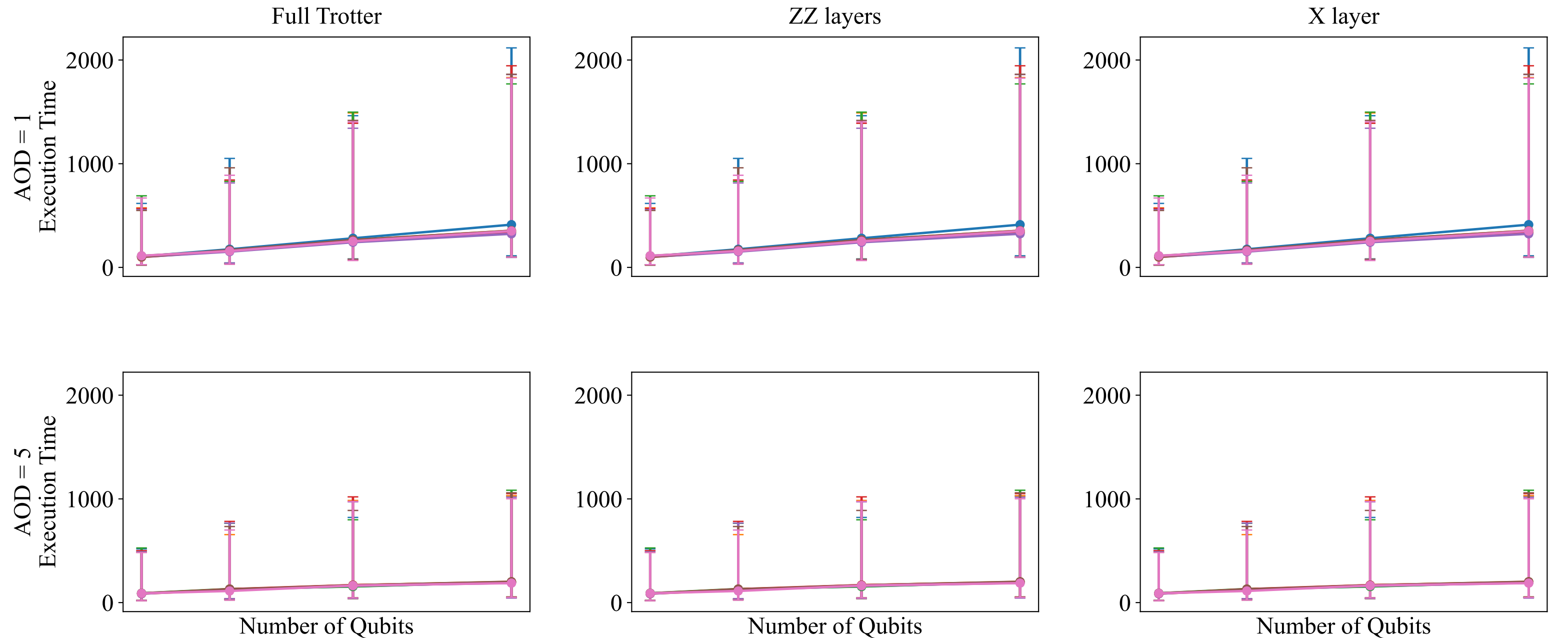
Ablation study (checkerboard) - Execution Time
