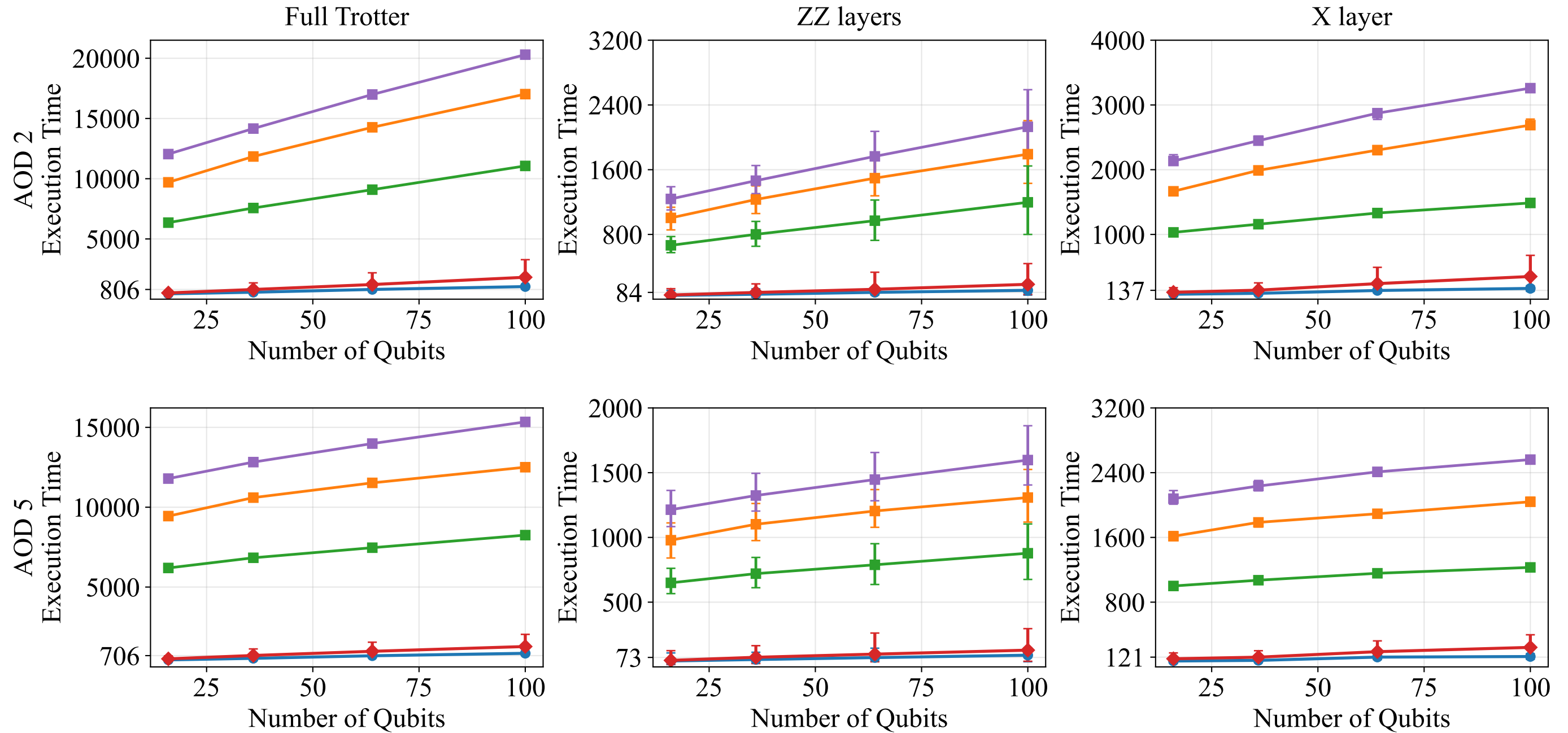
STAR vs T cultivation runtime · Columns: Full Trotter | ZZ layers | X layer · Rows: AOD 2 (top), AOD 5 (bottom)
