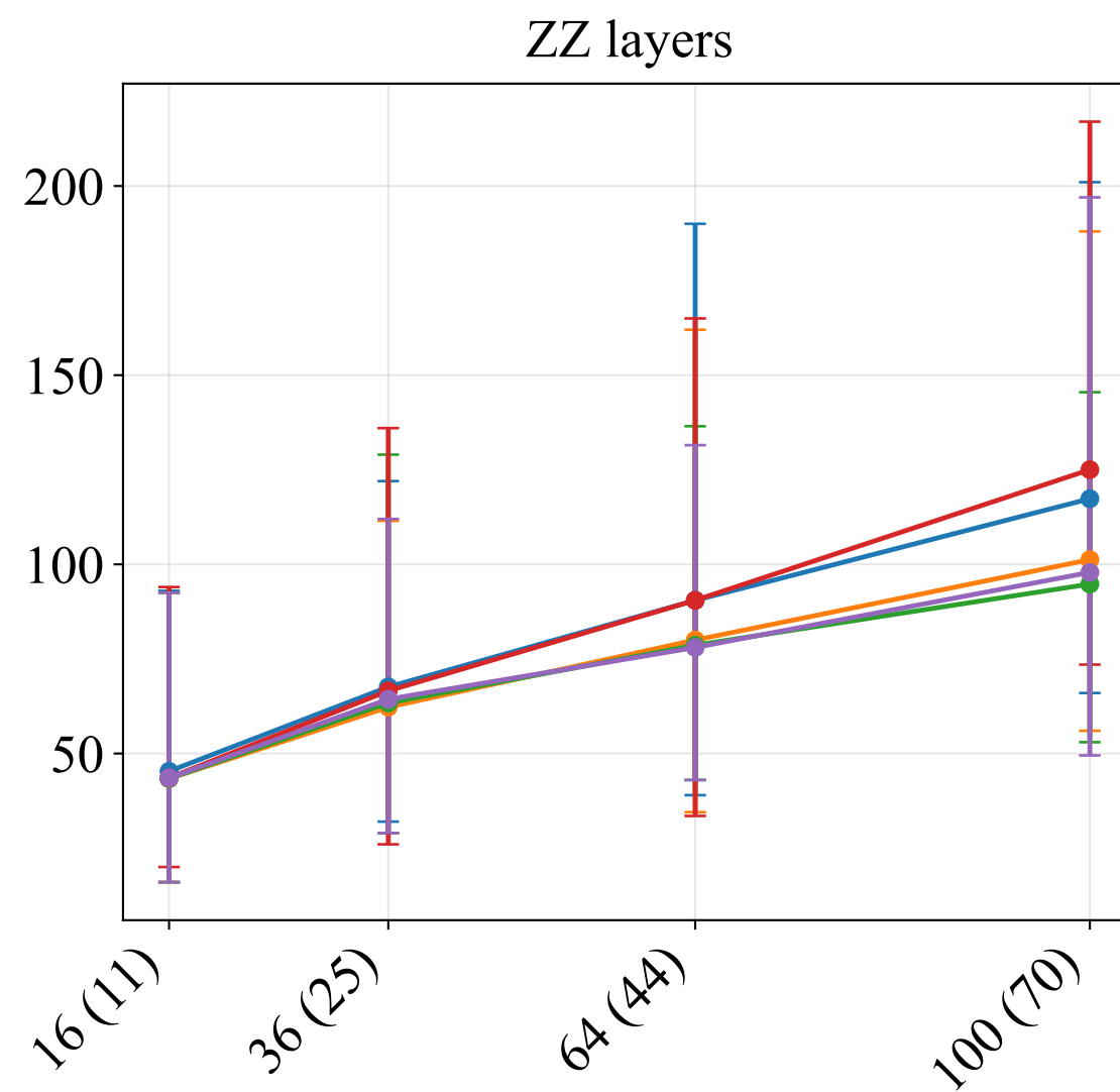
Ablation Study, Execution Time, distance=9
