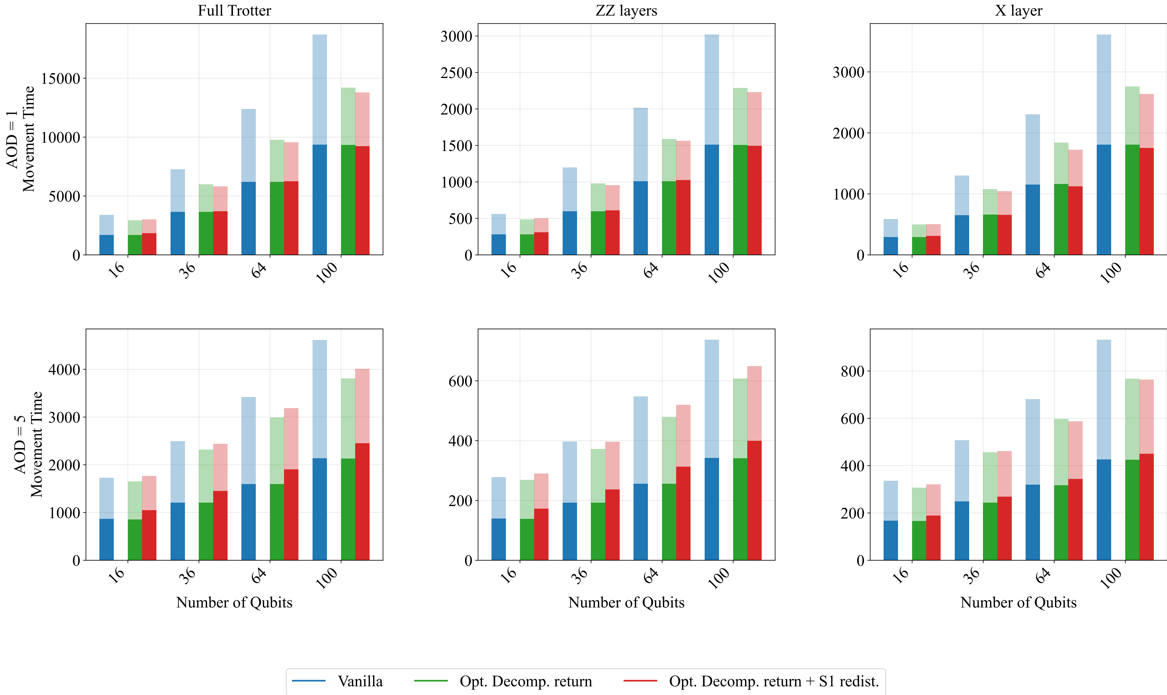
T-cultivation compile ablation (d=9), Movement Time (d=9)
