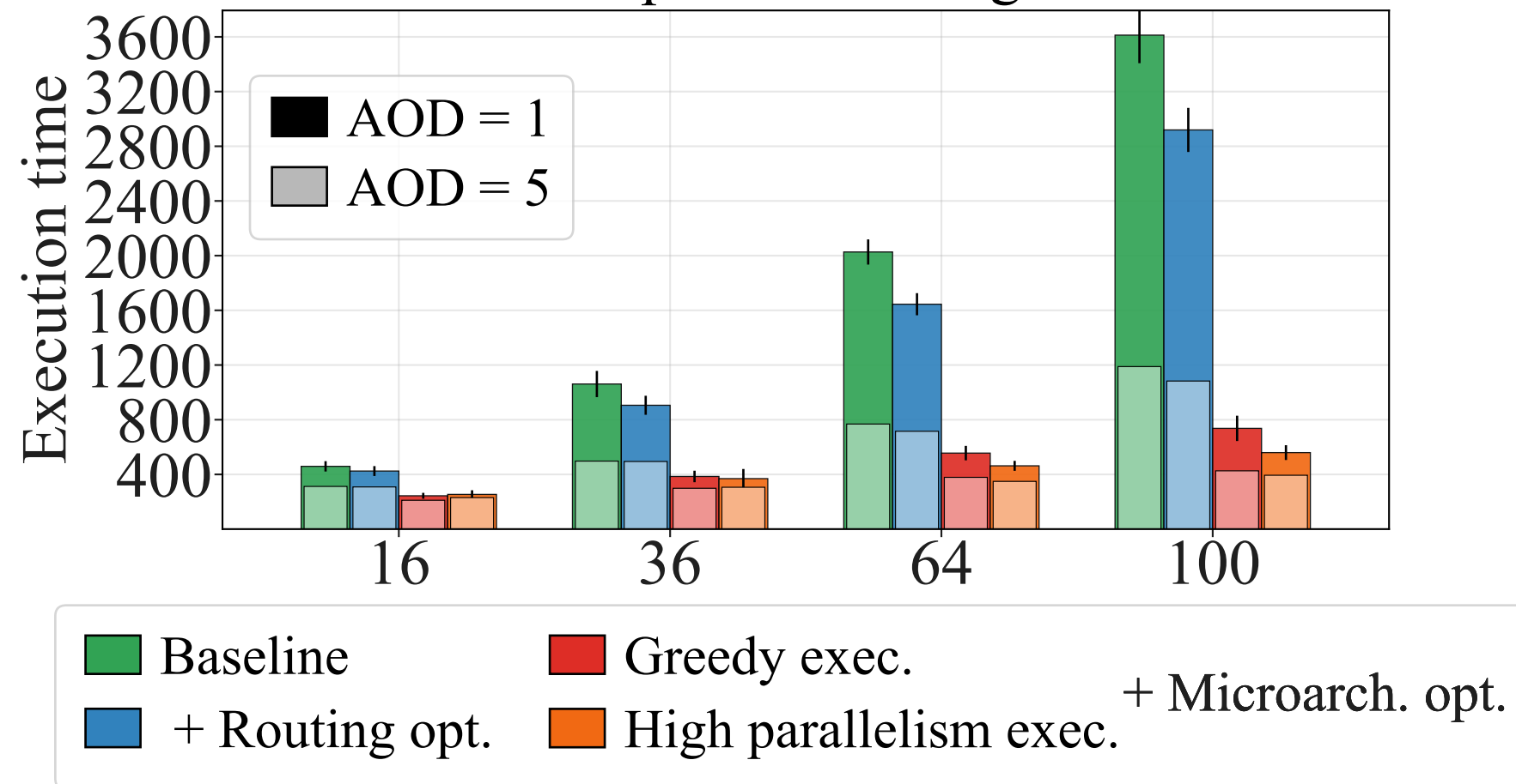
STAR architecture Compilation Strategies
