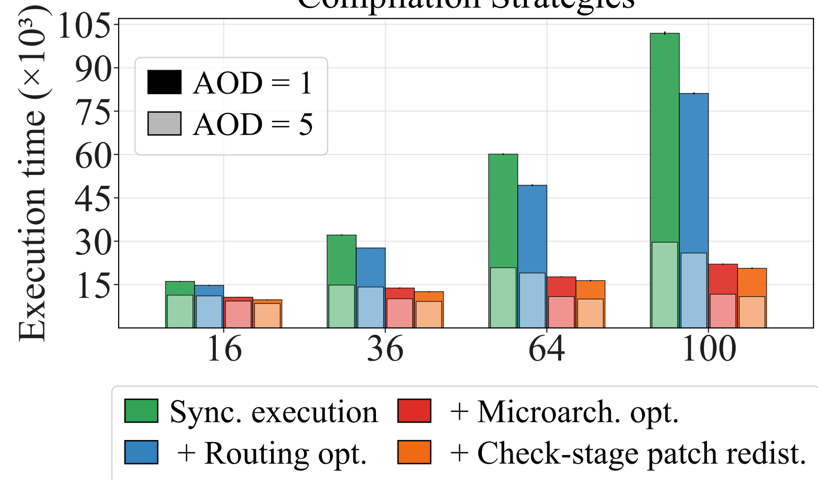
AOD comparison
