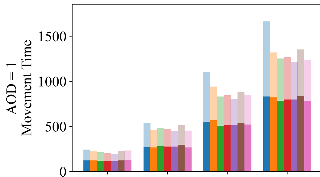
Full Trotter
