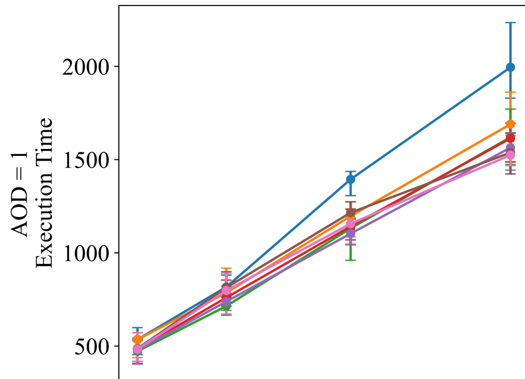
Full Trotter
