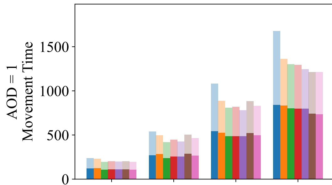
Full Trotter
