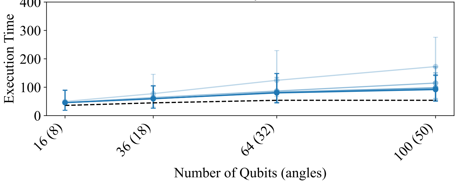
ZZ layers
