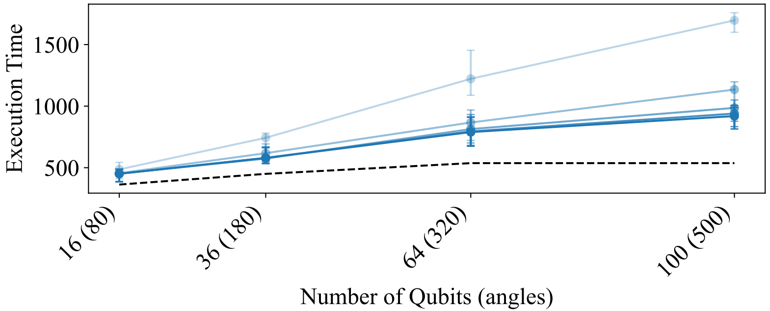
Full Trotter
