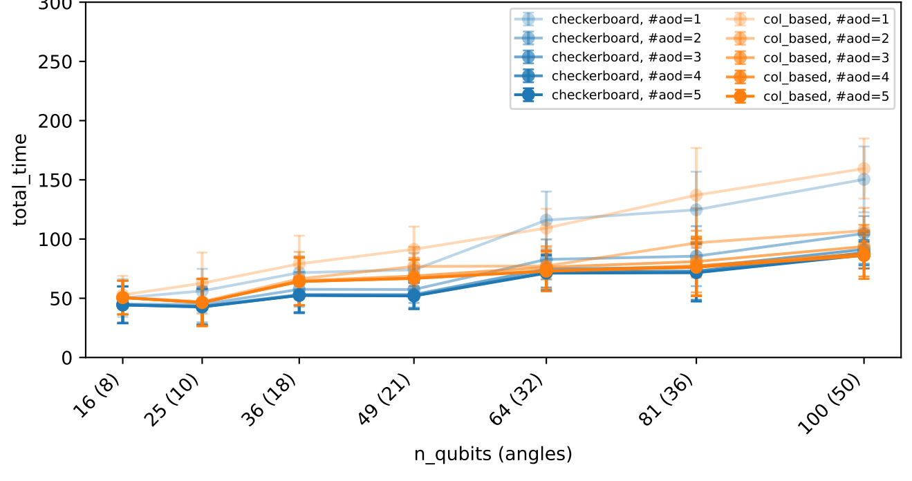
Total time for placement × #aod - round_1
