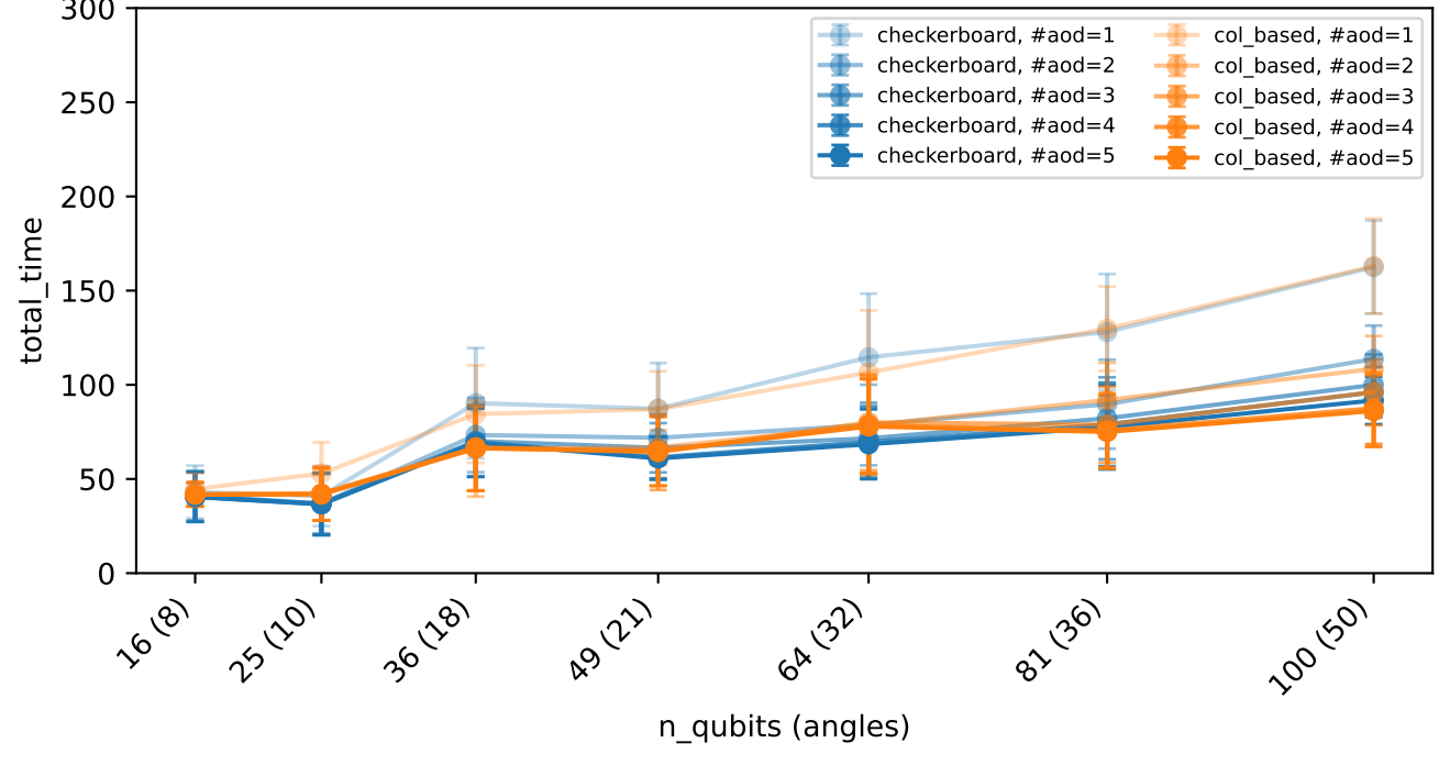
Total time for placement × #aod - round_3
