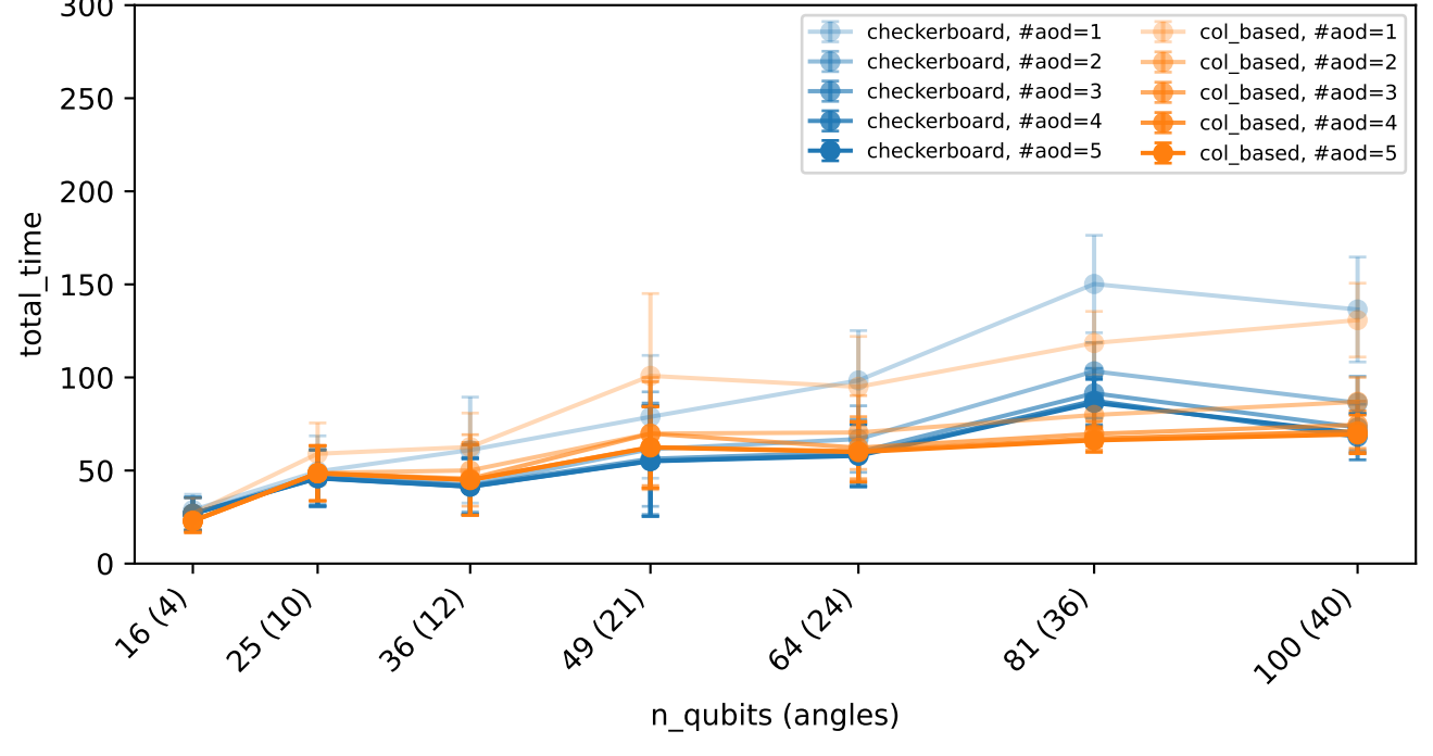
Total time for placement × #aod - round_2
