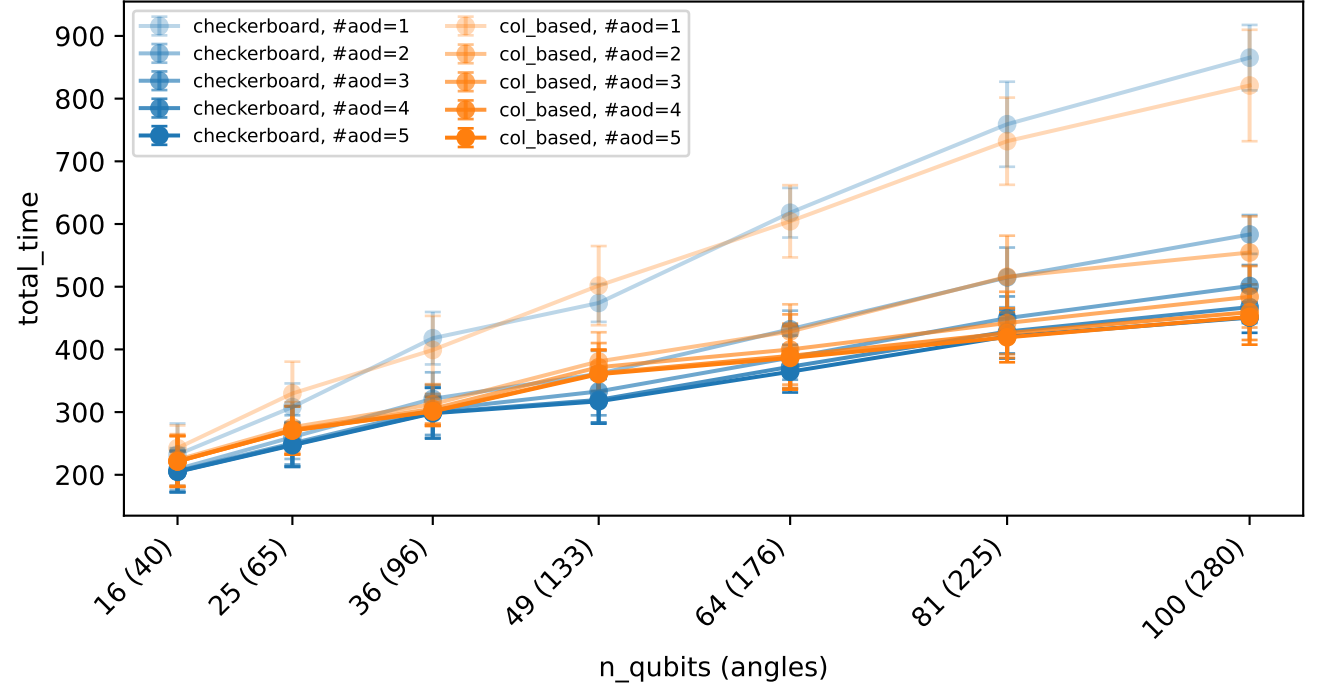
Total time for placement × #aod - round_0
