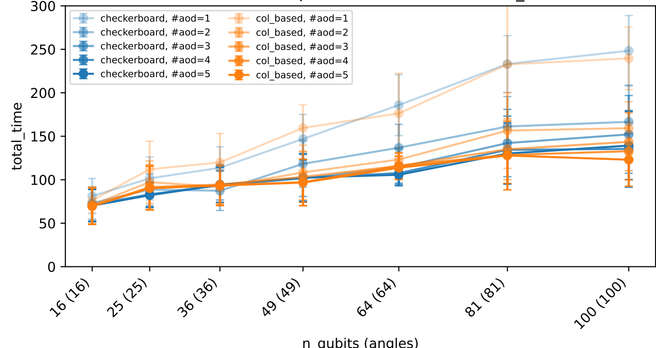
Total time for placement × #aod - round_4
