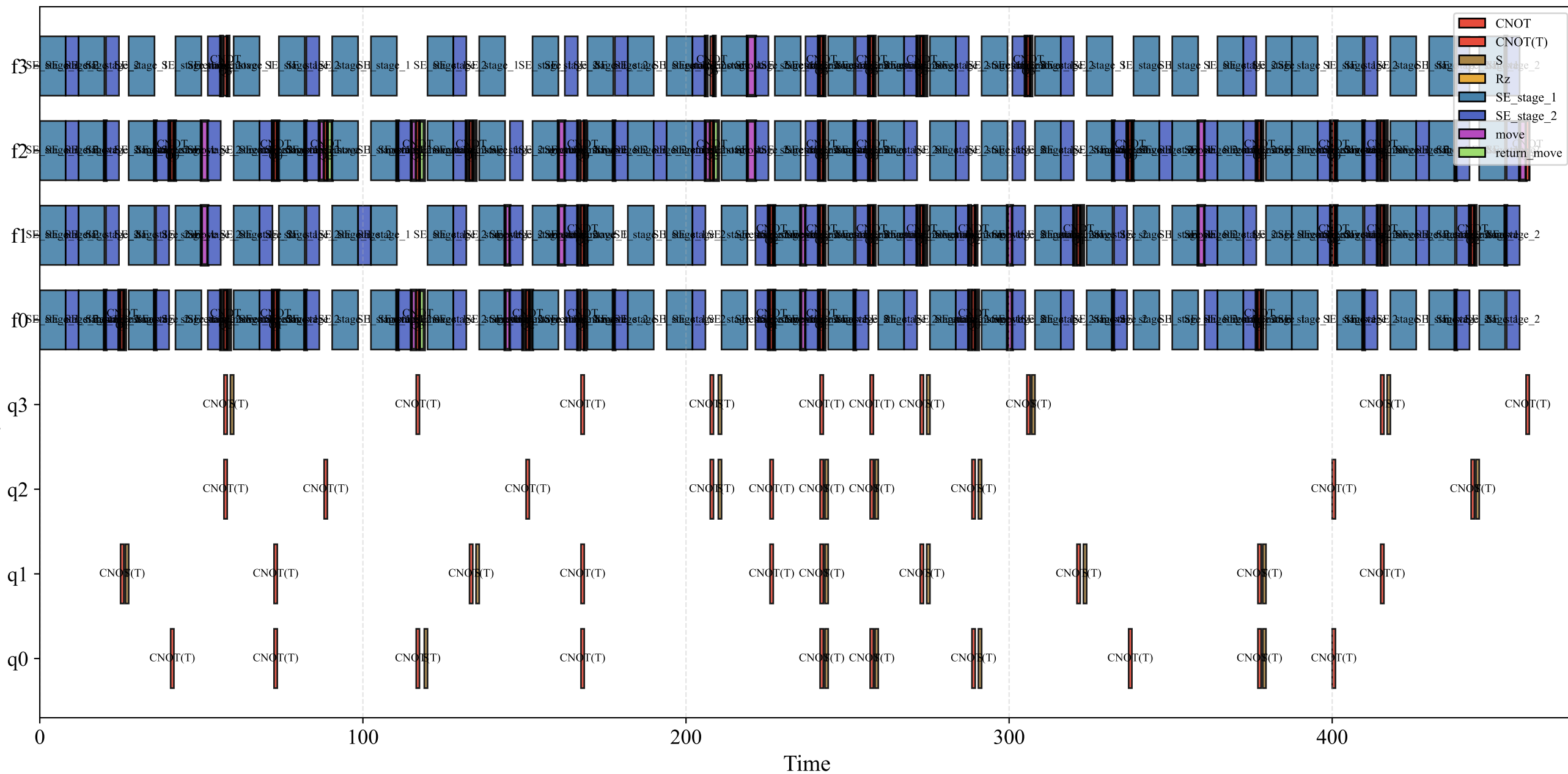
T-Cultivation Execution Time
