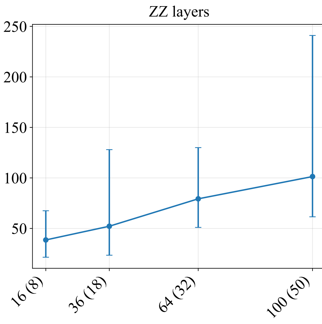
Ablation Study, Execution Time, distance=7
