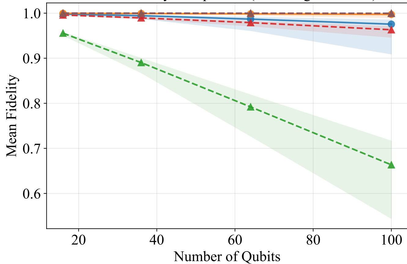
Overall Fidelity Comparison (Including Idle Error)
