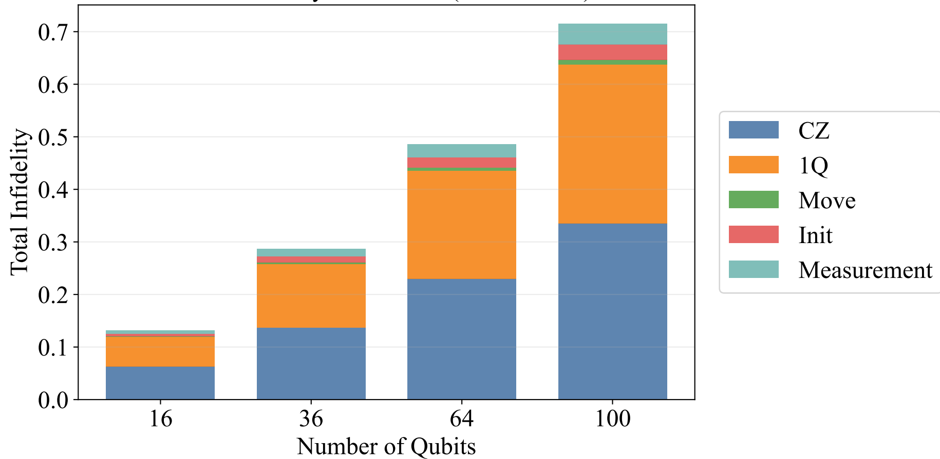
Raw Infidelity Breakdown (Without Idle)
